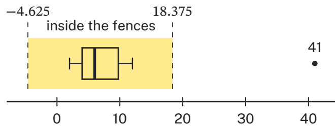
Figure 5. The running example, with type-7 quartiles, the two fences, observed whisker endpoints, and the single flagged value 41.
